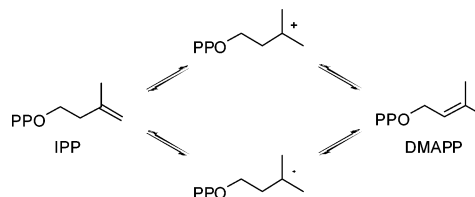
Scheme 2. Potential Reactions for Mechanism-Based Inhibition of IDI-2 by cIPP (X = CH 2 ) and oIPP (X = O)
