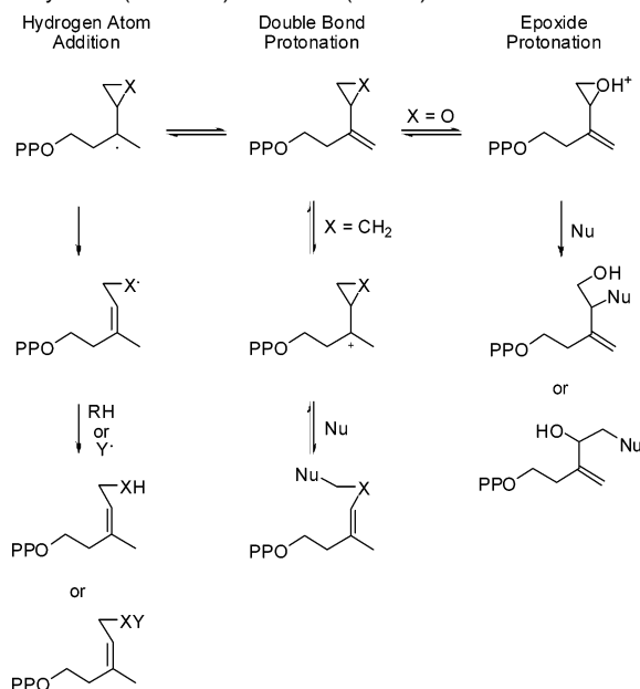
Scheme 2. Potential Reactions for Mechanism-Based Inhibition of IDI-2 by cIPP (X = CH 2 ) and oIPP (X = O)
